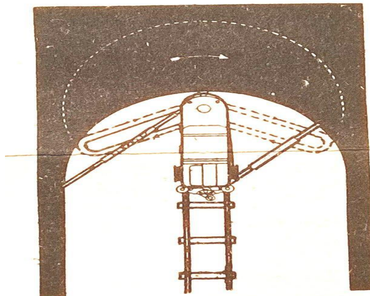
Fig. 8. Arcwalling.
