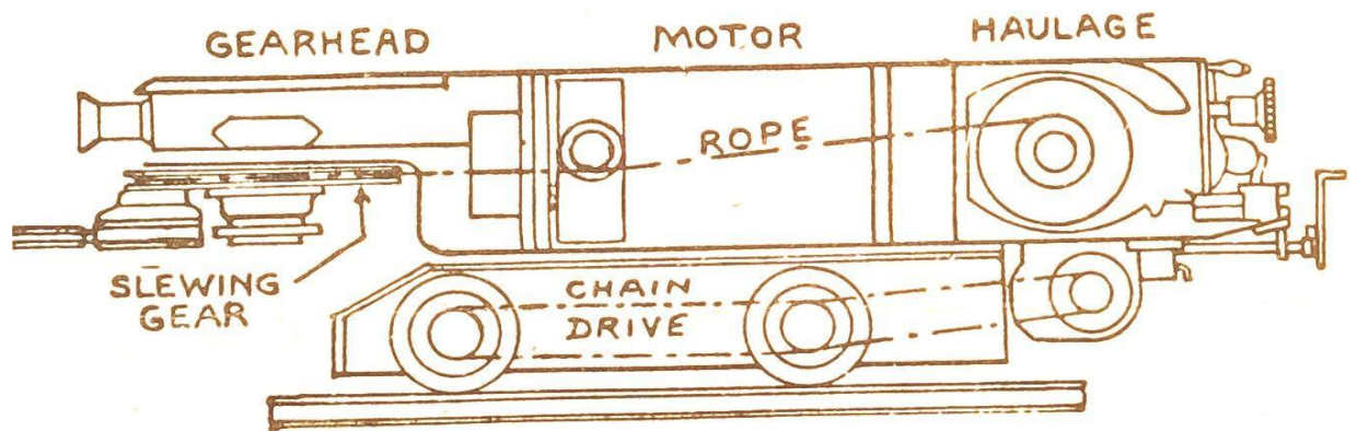
Fig. 7. Arcwall Coal-cutter. ( M. and C. Ltd. )
