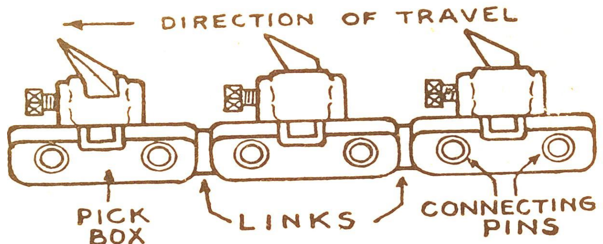
Fig. 2. Cutter Chain.
