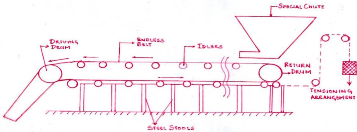
Arrangement of a belt conveyor
