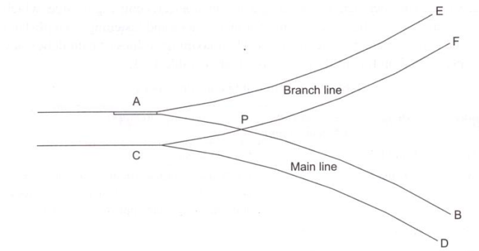
Fig: Negative superelevation
