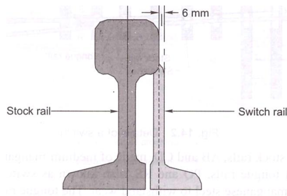
Fig. Undercut switch
