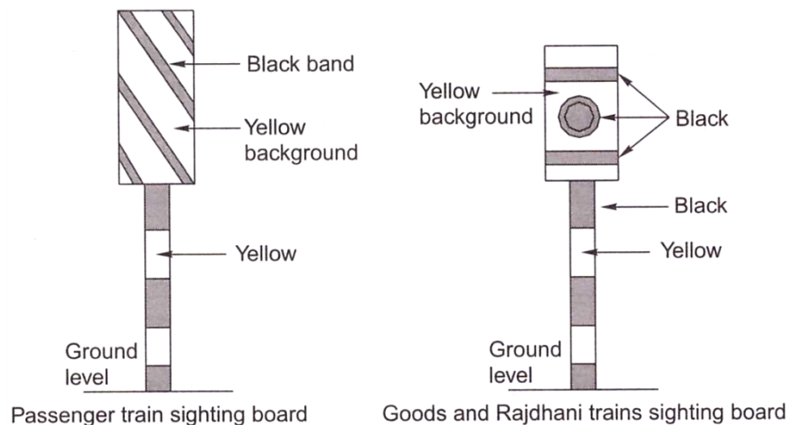
Fig. Sighting board
