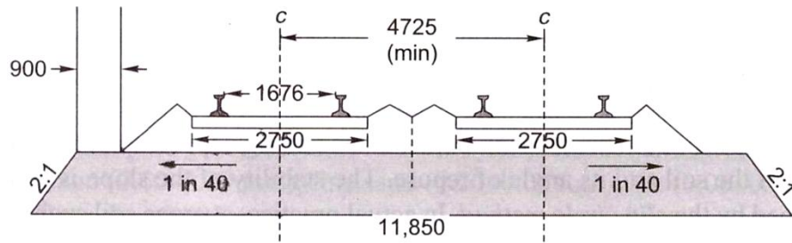
(a) Cross section of bank
