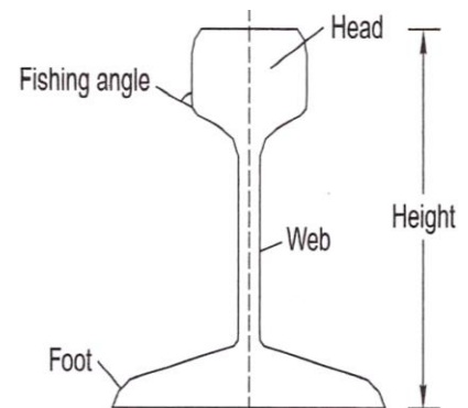
FLAT-FOOTED RAIL
