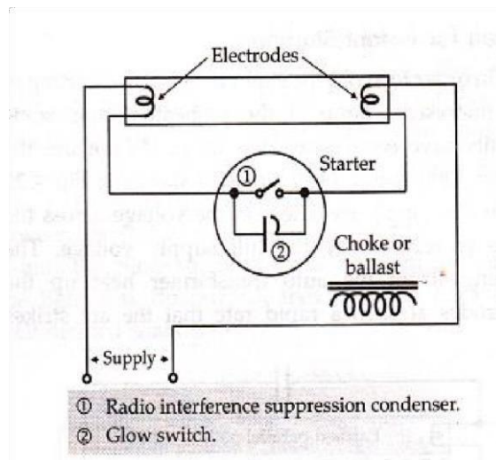
Fig.9 Fluorescent lamp
